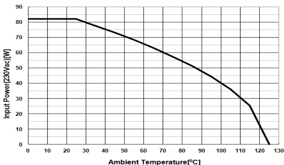
Figure 43: Input power curve V_{in}=230\text{Vac} ; P_{in}=f(T_a)
