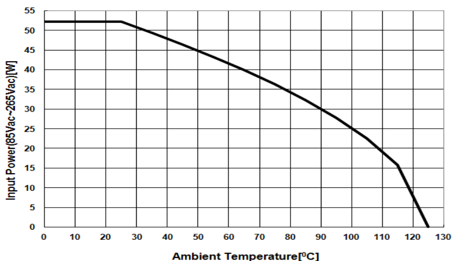
Figure 42: Input power curve V_{in}=85\sim 265\text{Vac} ; P_{in}=f(T_a)
