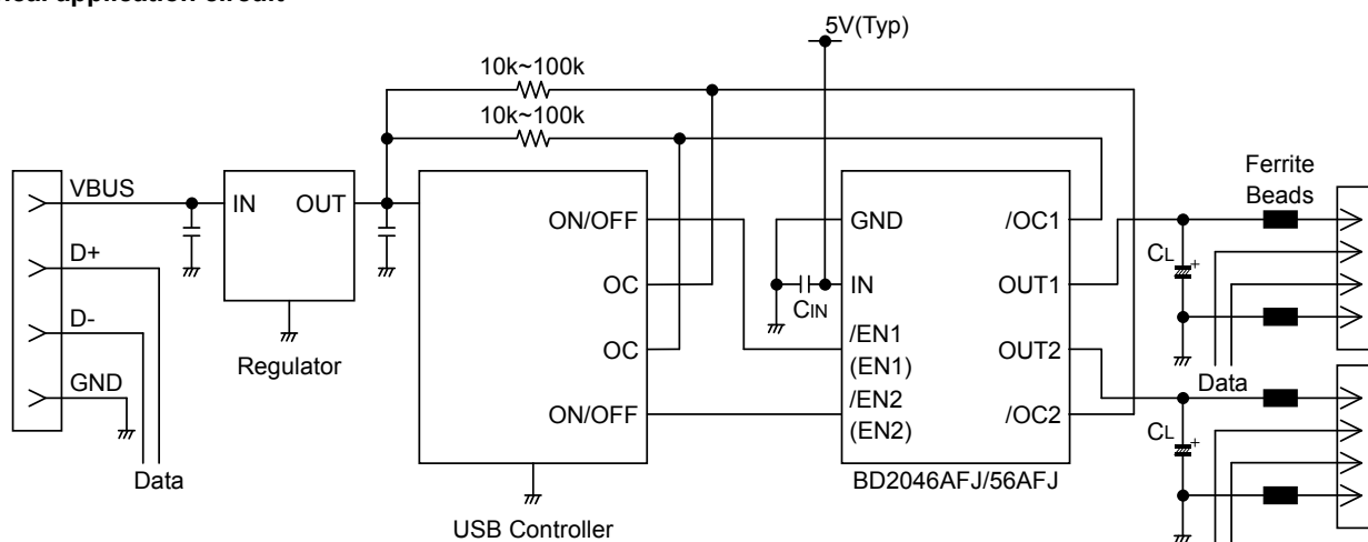
Fig.40 Typical application circuit
