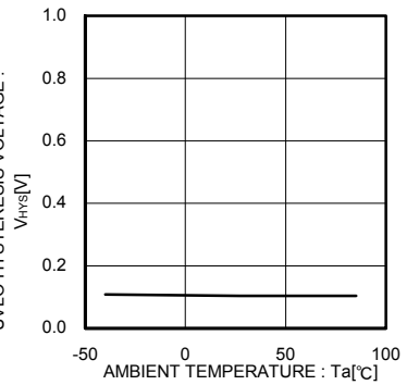
Fig.25 UVLO hysteresis voltage
