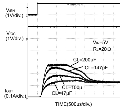
Fig.28 Inrush current response (BD2056AFJ)
