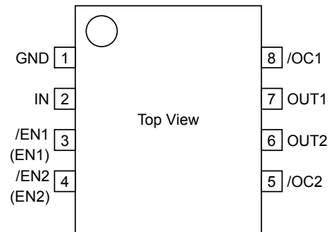
Fig.37 Pin Configuration
