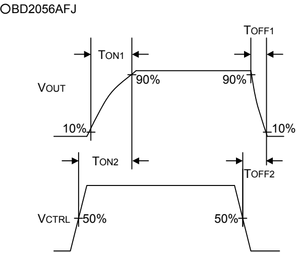
Fig.3 Timing diagram
