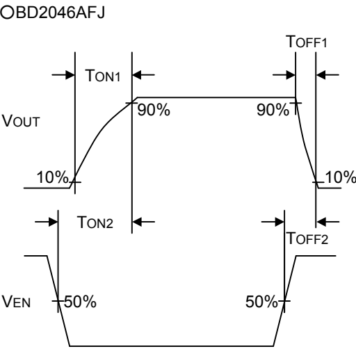
Fig.2 Timing diagram
