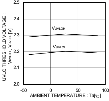
Fig.24 UVLO threshold voltage
