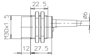
E2EL-X15M□-L 2M
