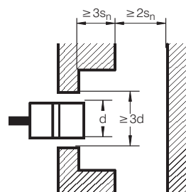
Fig.3: Non-shielded type
