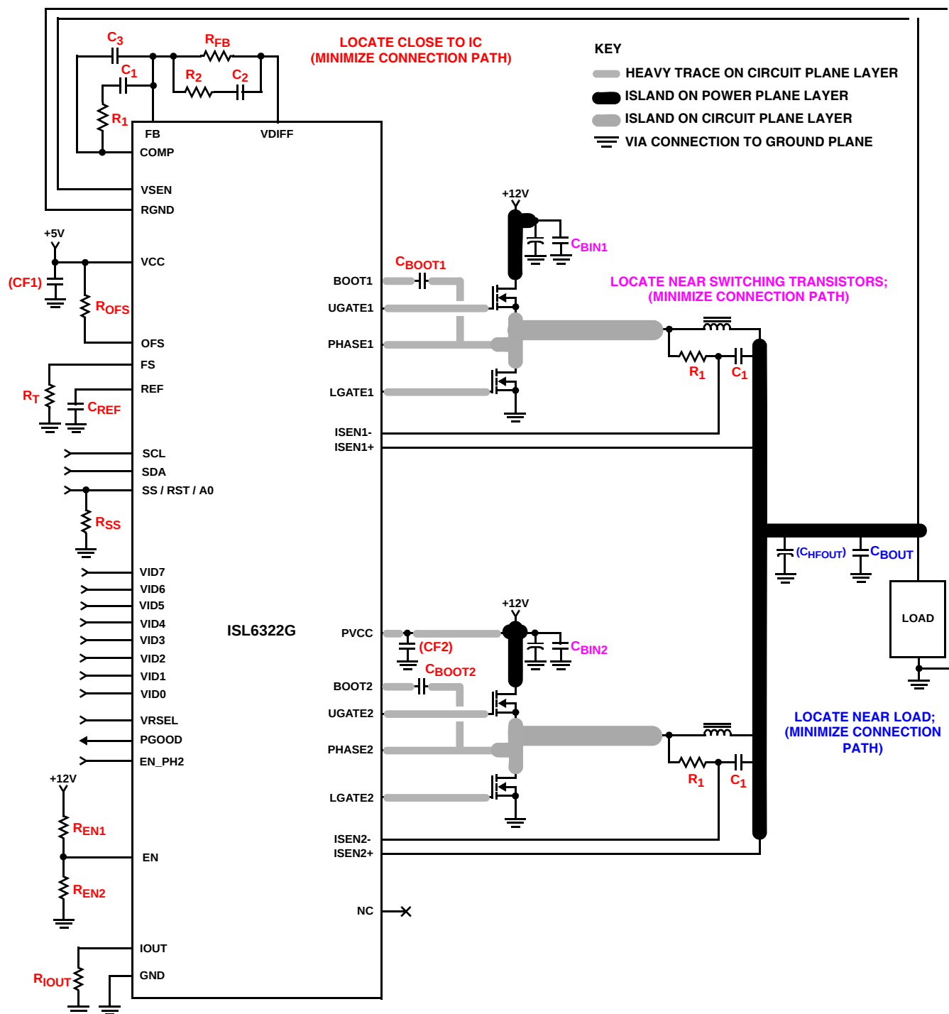
FIGURE 26. PRINTED CIRCUIT BOARD POWER PLANES AND ISLANDS
