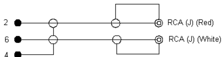
Wiring Diagram
