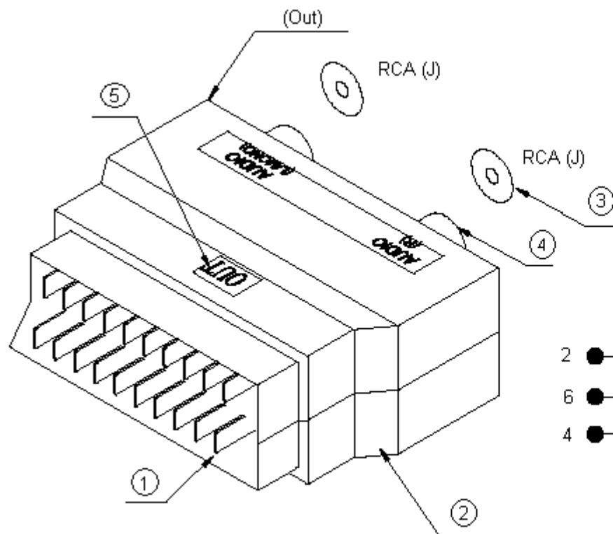
21 Pin (P)/2RCA (J) Converter
