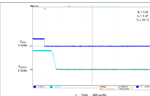
Figure 6-12. Turnoff Delay and Fall Time With 1-μF Load
