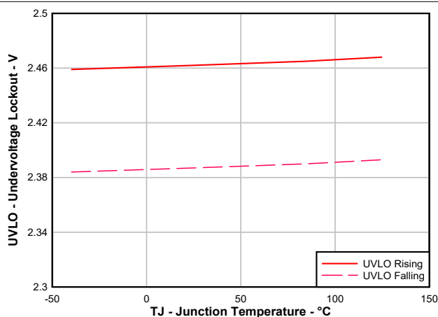
Figure 6-9. Undervoltage Lockout vs Junction Temperature
