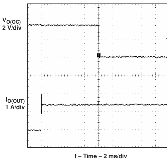
Figure 6-37. 1-Ω Load Connected to Enabled Device
