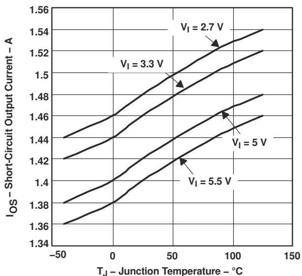
Figure 6-26. SHORT-CIRCUIT OUTPUT CURRENT vs JUNCTION TEMPERATURE
