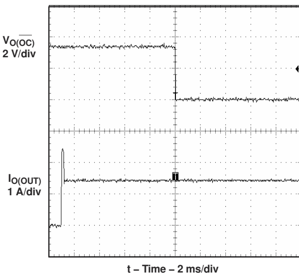
Figure 6-36. 2-Ω Load Connected to Enabled Device
