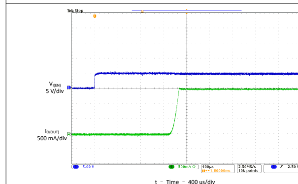
Figure 6-15. Short-Circuit Current, Device Enabled Into Short
