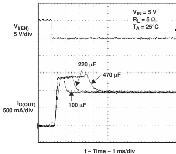
Figure 6-35. Inrush Current With Different Load Capacitance
