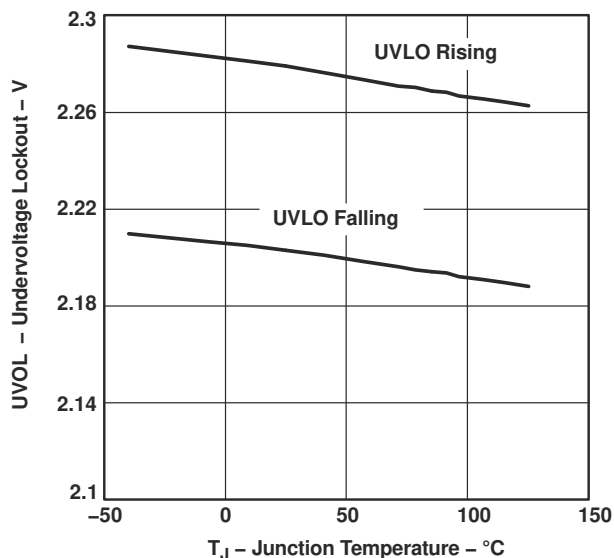
Figure 6-28. UNDERVOLTAGE LOCKOUT vs JUNCTION TEMPERATURE
