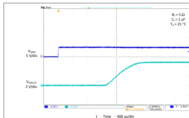
Figure 6-11. Turnon Delay and Rise Time With 1-μF Load
