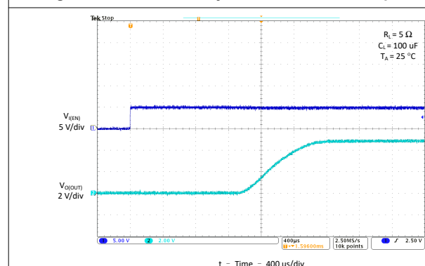
Figure 6-13. Turnon Delay and Rise Time With 100-μF Load
