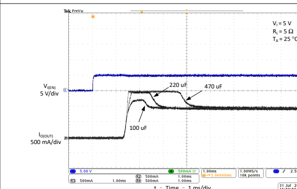
Figure 6-16. Inrush Current With Different Load Capacitance
