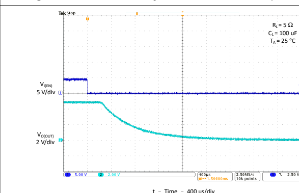
Figure 6-14. Turnoff Delay and Fall Time With 100-μF Load
