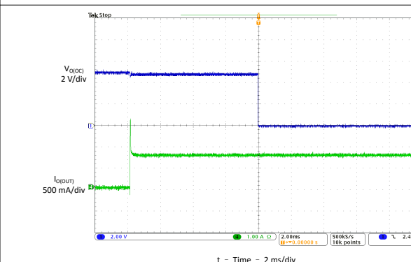
Figure 6-18. 2-Ω Load Connected to Enabled Device
