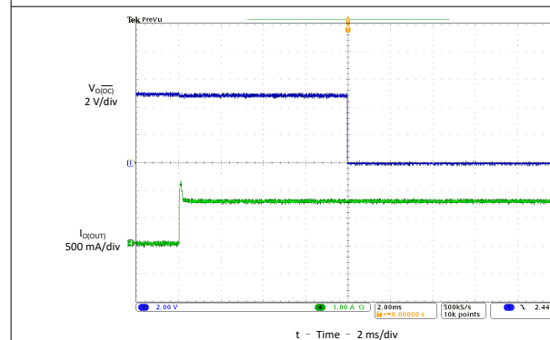
Figure 6-17. 3-Ω Load Connected to Enabled Device
