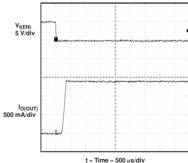
Figure 6-34. Short-Circuit Current, Device Enabled Into Short
