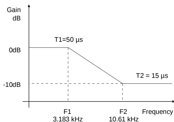
Figure 27. De-Emphasis Curve
