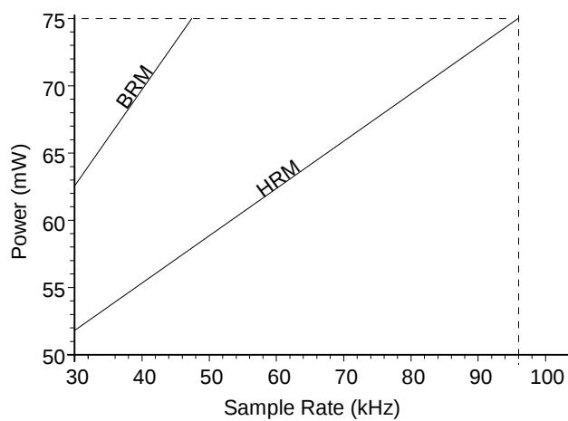
Figure 19. Power vs. Sample Rate ( V_A = 5V )
