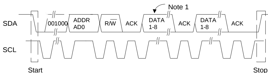
Figure 8. I 2 C Mode Control Port Forming
