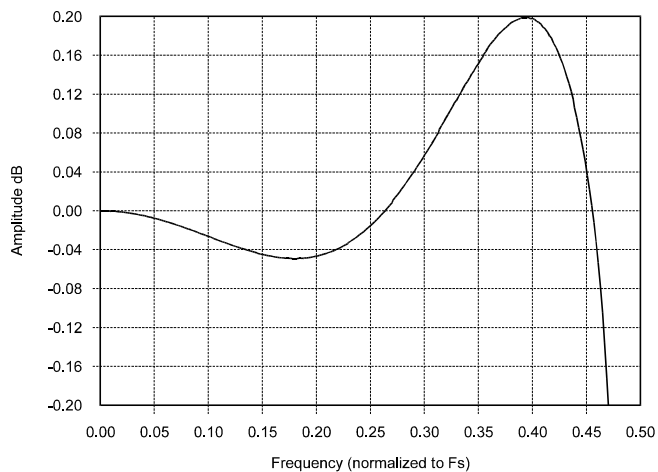
Figure 16. High-Rate Passband Ripple
