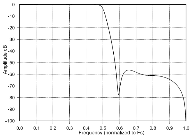
Figure 13. High-Rate Stopband Rejection
