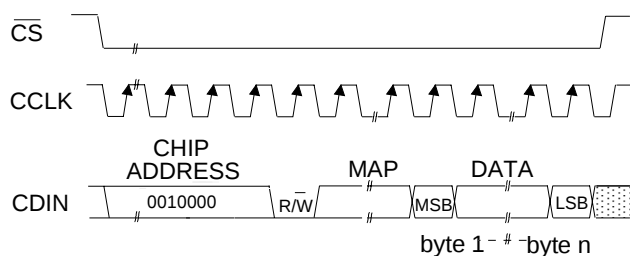
Figure 7. SPI Mode Control Port Forming
