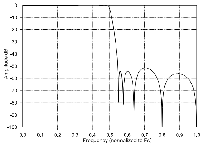
Figure 9. Base-Rate Stopband Rejection
