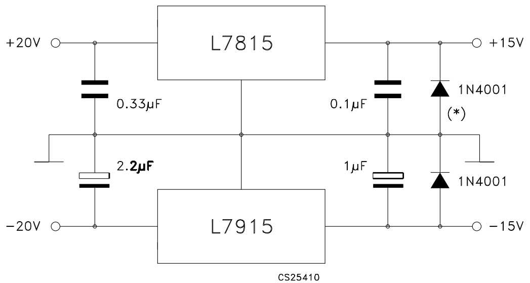
Figure 17. Split power supply ( \pm 15 V - 1 A )
