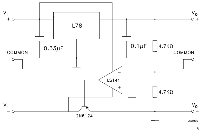
Figure 17. Split power supply ( \pm 15 V - 1 A )
