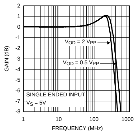
Figure 2. Frequency Response
