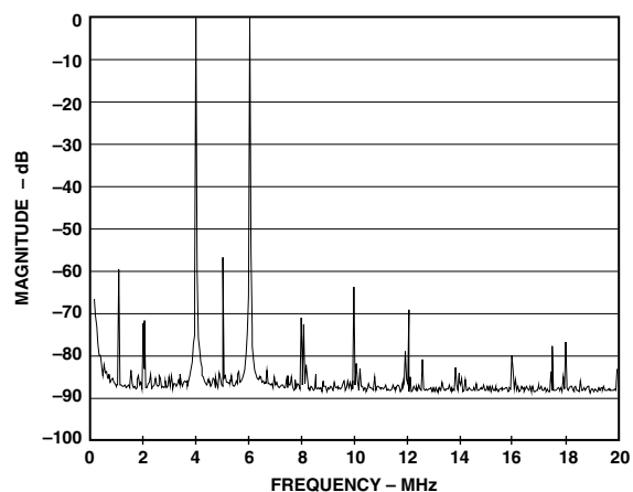
TPC 3b. Dual Sideband Spectral Plot, f_c = 5\text{ MHz} f = 1\text{ MHz} , R_{SET} = 4\text{ k}\Omega ( I_{OUT} = 10\text{ mA} ), RBW = 1 kHz
