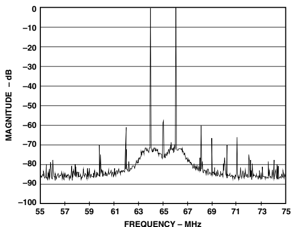
TPC 4a. Dual Sideband Spectral Plot, f_c = 65\text{ MHz} f = 1\text{ MHz} , R_{SET} = 10\text{ k}\Omega ( I_{OUT} = 4\text{ mA} ), RBW = 1 kHz
