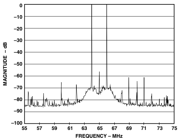
TPC 4b. Dual Sideband Spectral Plot, f_c = 65\text{ MHz} f = 1\text{ MHz} , R_{SET} = 4\text{ k}\Omega ( I_{OUT} = 10\text{ mA} ), RBW = 1 kHz
