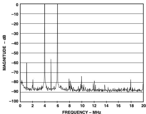
TPC 3a. Dual Sideband Spectral Plot, f_c = 5\text{ MHz} f = 1\text{ MHz} , R_{SET} = 10\text{ k}\Omega ( I_{OUT} = 4\text{ mA} ), RBW = 1 kHz
