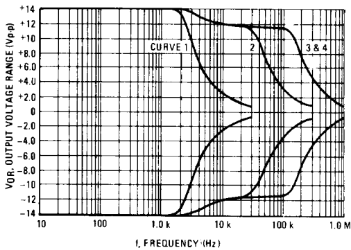
FIGURE 4 – LARGE SIGNAL SWING versus FREQUENCY
