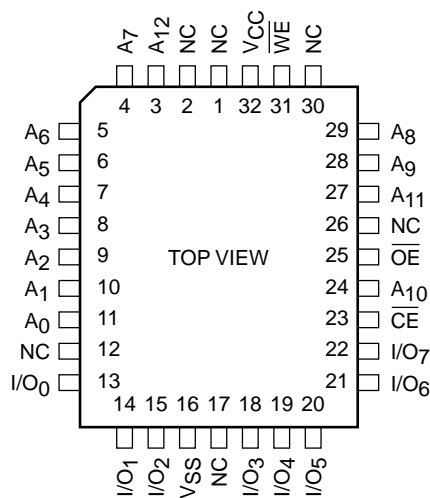
PLCC Package (N)
