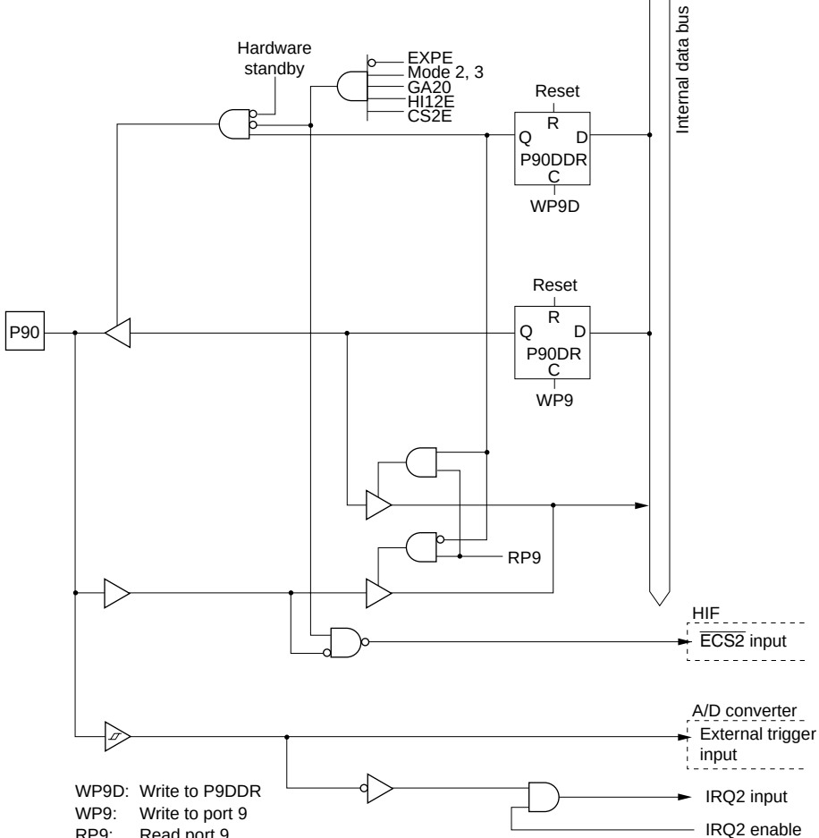
Figure C.29 Port 9 Block Diagram (Pin P90)
