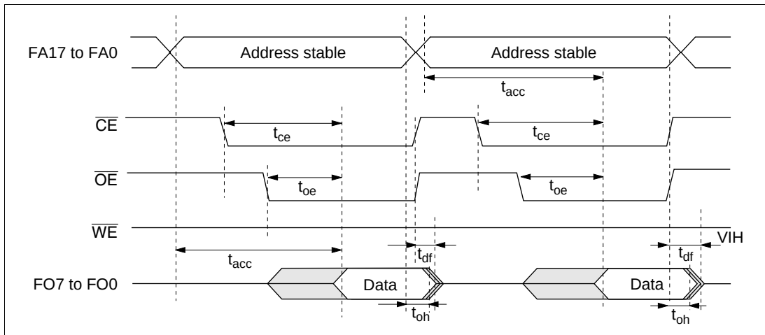
Figure 21.19 Timing Waveforms for \overline{\text{CE}}/\overline{\text{OE}} Clocked Read
