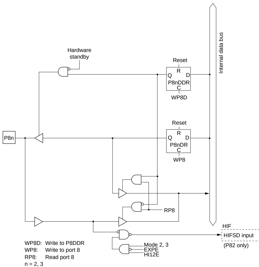
Figure C.25 Port 8 Block Diagram (Pins P82, P83)
