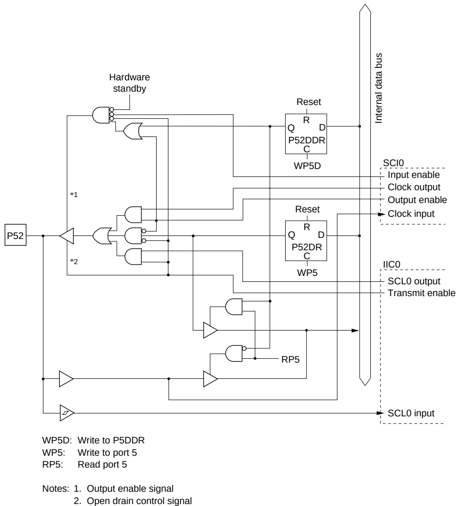
Figure C.15 Port 5 Block Diagram (Pin P52)
