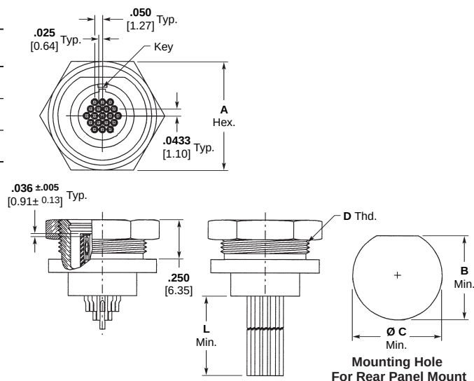
Rear Panel Mount (19 Position Shown)
