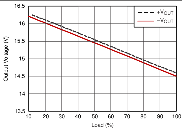
Figure 6-26. Load Regulation
