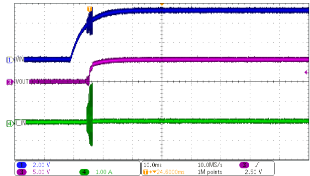
Figure 7-4. DCP010505BP Start-Up at 10% Load
