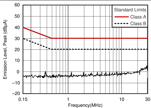
Figure 6-2. Conducted Emissions
