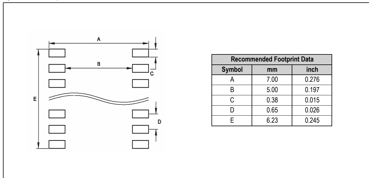
Figure 20. PCB Footprint
