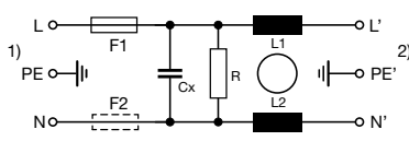
Medical version (M5) without voltage selector
