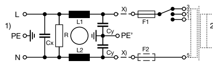
Medical version (M80) with voltage selector
