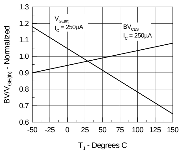
Fig. 6. Temperature Dependence of BV_{CES} & V_{GE(th)}
