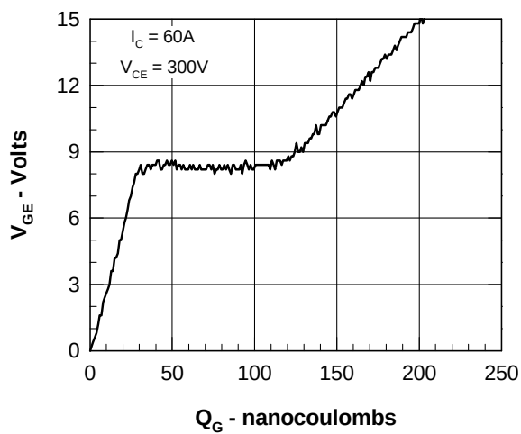
Fig. 9. Gate Charge
