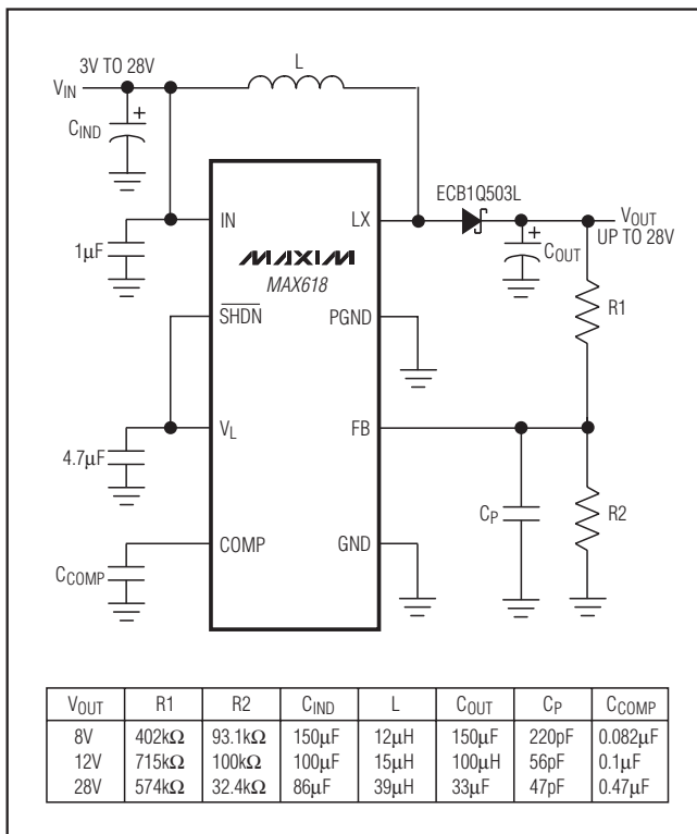
Figure 1. Single-Supply Operation
