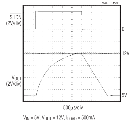
SHUTDOWN RESPONSE
