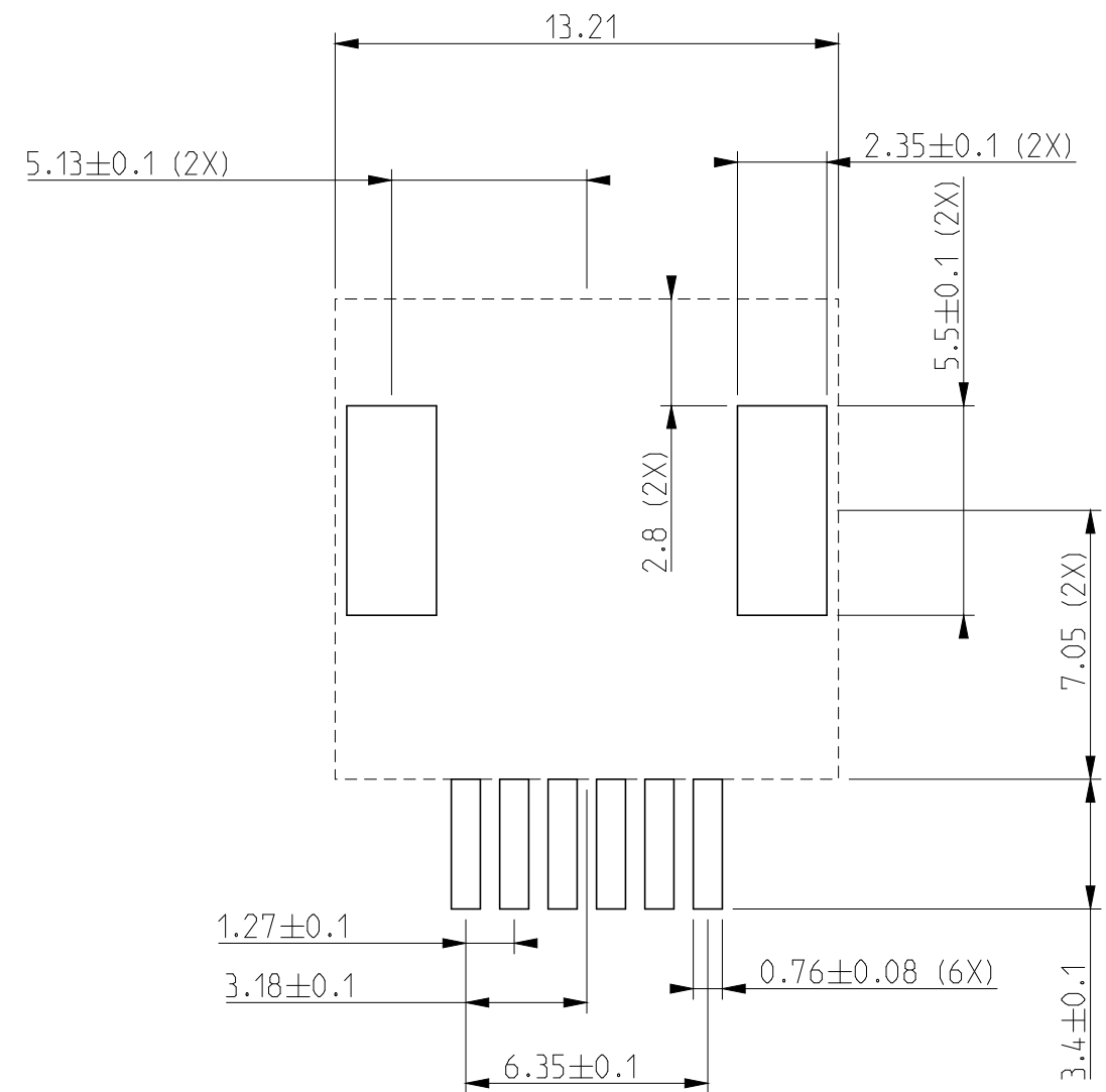
RECOMMENDED PCB FOOT PRINT FOR 6 POSITIONS INSIDE
