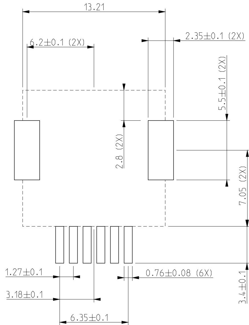
RECOMMENDED PCB FOOT PRINT FOR 6 POSITIONS OUTSIDE
