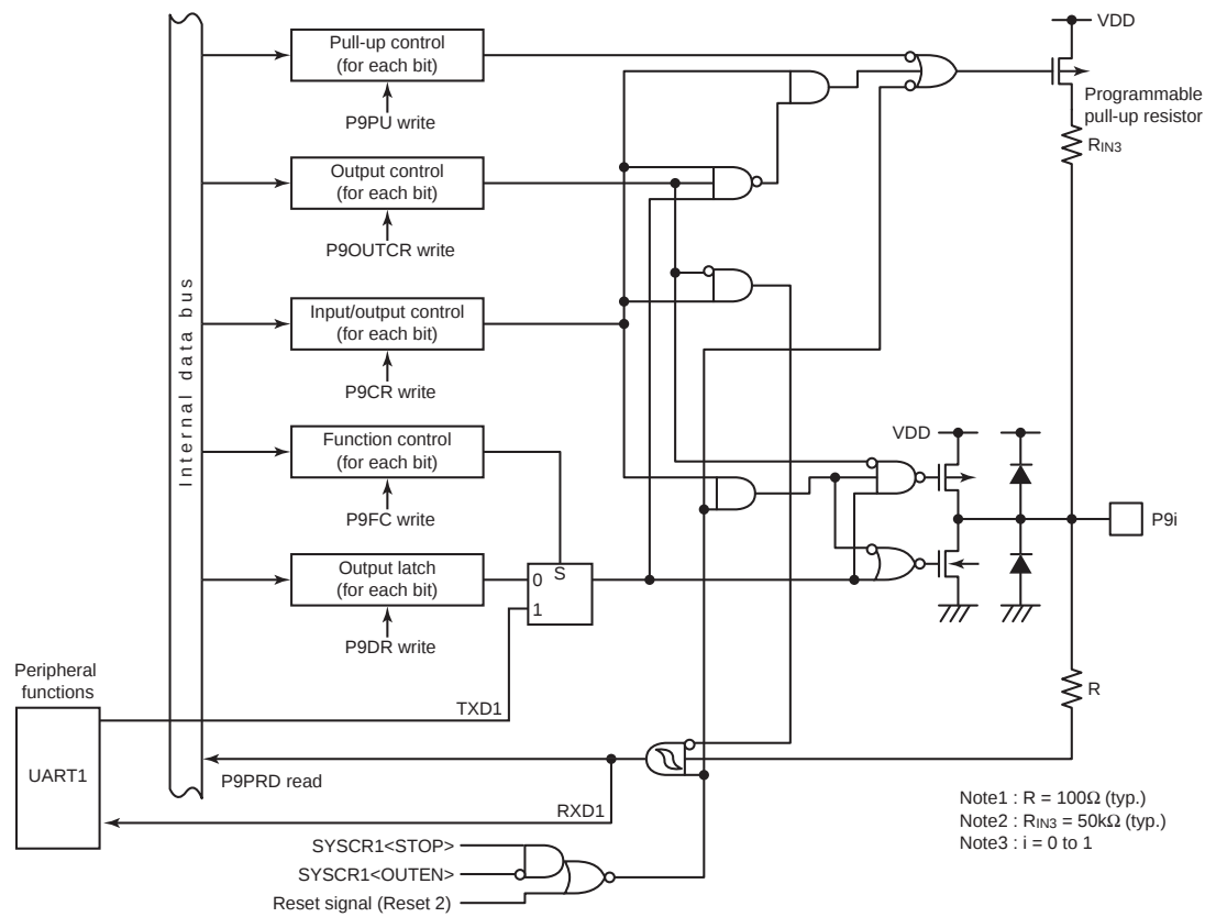
Figure 8-9 Port P9
