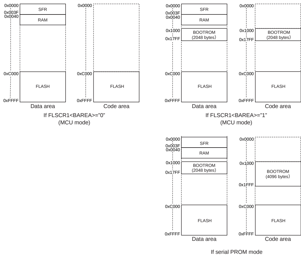
Figure 22-3 Memory Mapping
