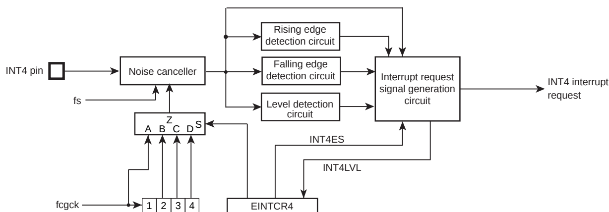
Figure 4-3 External Interrupt 4
