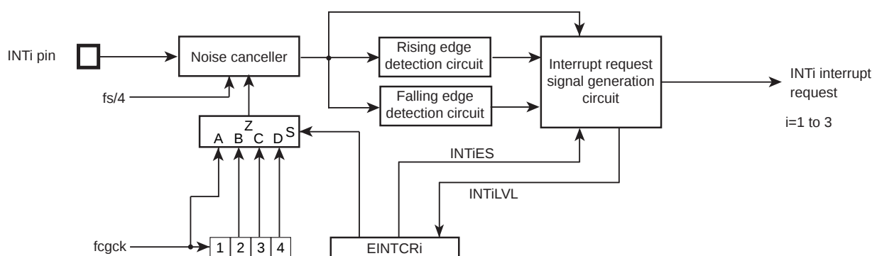
Figure 4-2 External Interrupts 1/2/3
