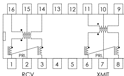
SCHEMATIC DIAGRAM "H"
