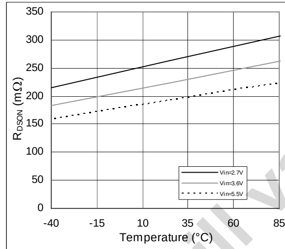
Figure 20. R_{DS(on)} (N-Channel) vs. Temp.; I_{SW}=200\text{mA}
