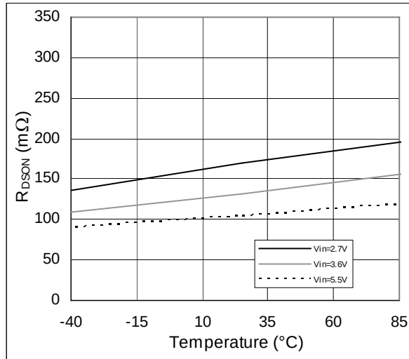
Figure 19. R_{DS(on)} (P-Channel) vs. Temp.; I_{SW}=200\text{mA}
