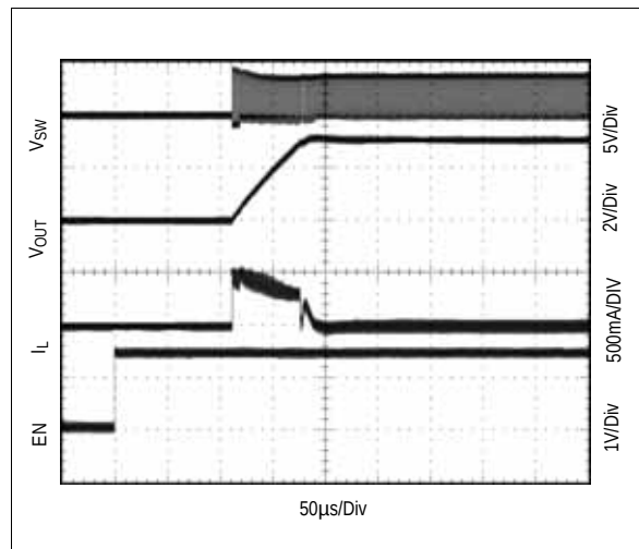
Figure 12. Startup; V_{IN} = 4.2V , V_{OUT} = 3.0V , I_{OUT} < 1mA , R_{LOAD} = 3.3k\Omega
