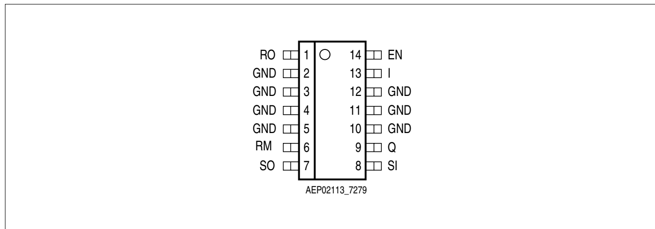
Figure 1 Pin Configuration
