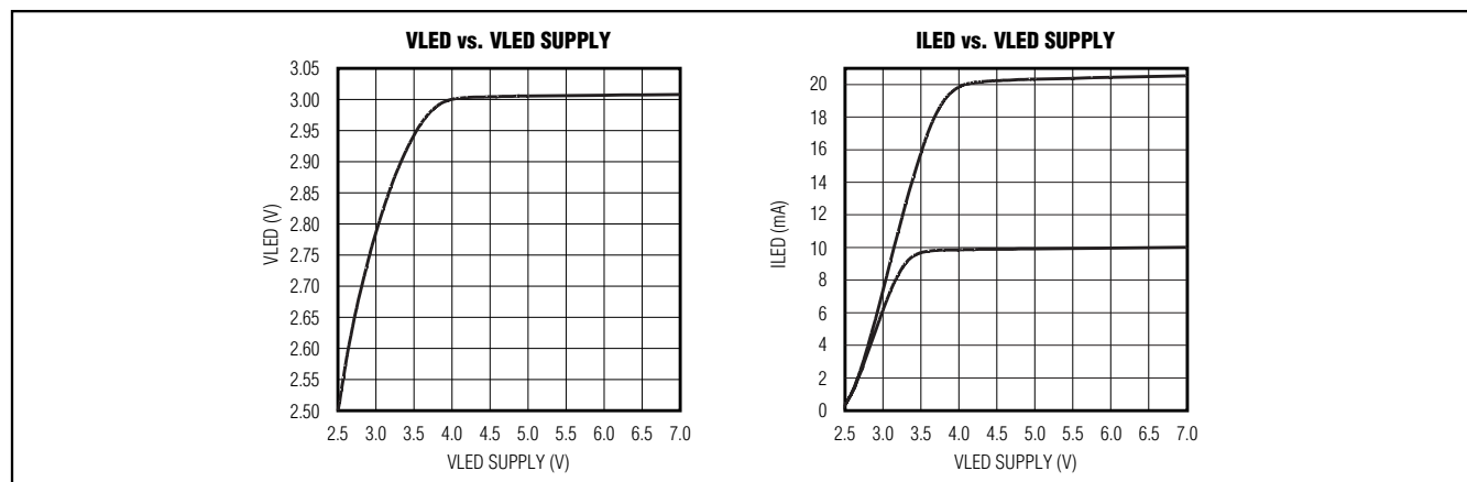
Figure 13. LED Brownout
