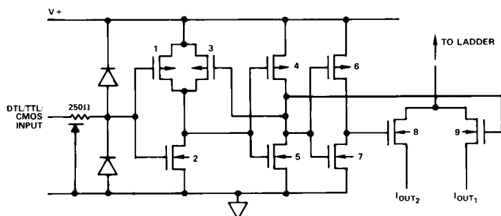
Figure 2. CMOS Switch
