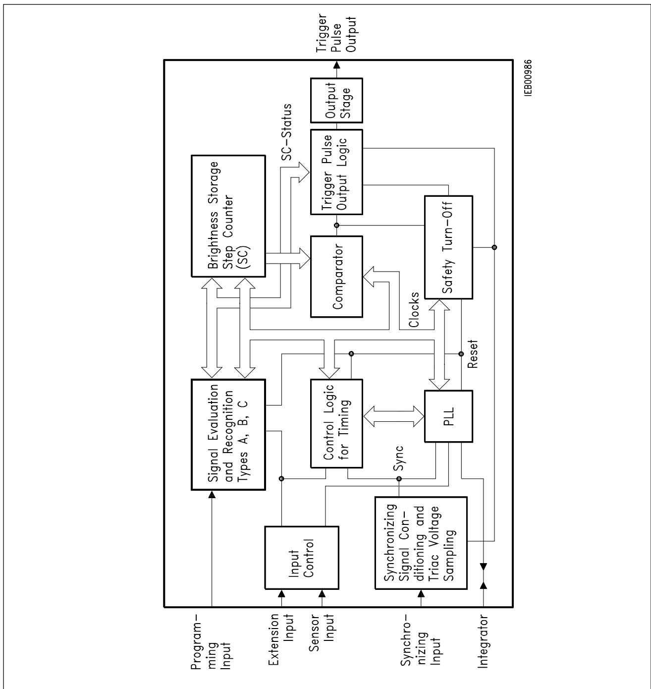
Figure 1 Block Diagram
