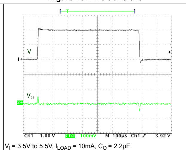
Figure 18. Line transient
