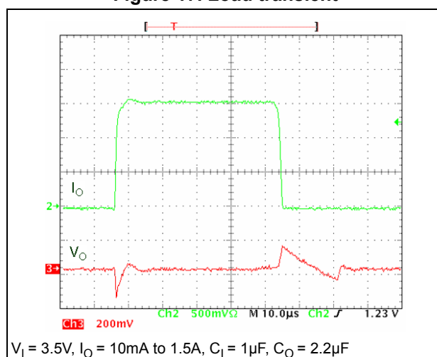
Figure 17. Load transient
