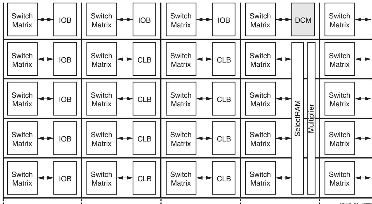
Figure 48: Routing Resources
