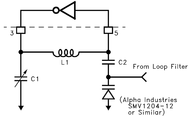
FIGURE 12. TYPICAL LC VCO
