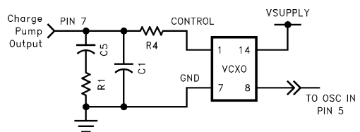
FIGURE 18. VCXO
