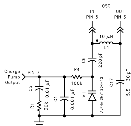
FIGURE 20. LC TANK
