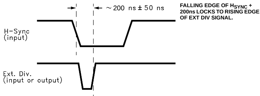
FIGURE 1. PLL LOCKED CONDITION (PHASE ERROR = 0)
