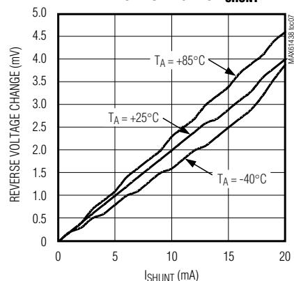
MAX6138_50 REVERSE VOLTAGE vs. I_{SHUNT}
