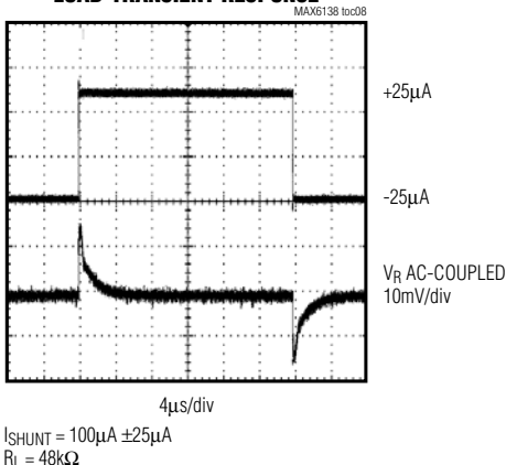
MAX6138_12 LOAD-TRANSIENT RESPONSE
