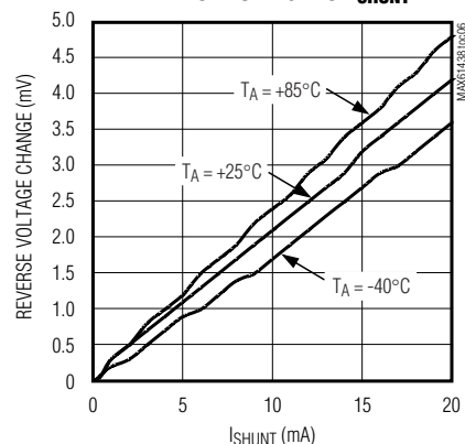
MAX6138_25 REVERSE VOLTAGE vs. I_{SHUNT}
