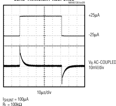
MAX6138_25 LOAD-TRANSIENT RESPONSE
