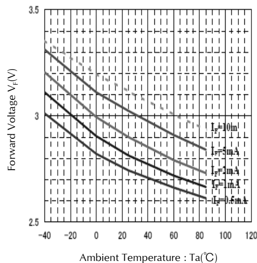
Ambient Temperature vs. Forward Voltage Condition : I_F = 0.5 \sim 10\text{mA}
