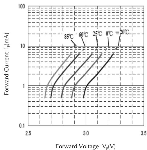
Forward Voltage vs. Forward Current Condition : T_a = -20^\circ\text{C} \sim 85^\circ\text{C}
