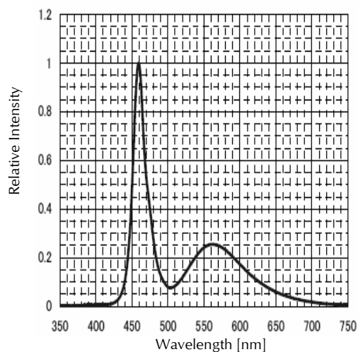
Spectral Distribution Relative Intensity vs. Wavelength Condition : T_a = 25^\circ\text{C} , I_F = 1\text{mA}
