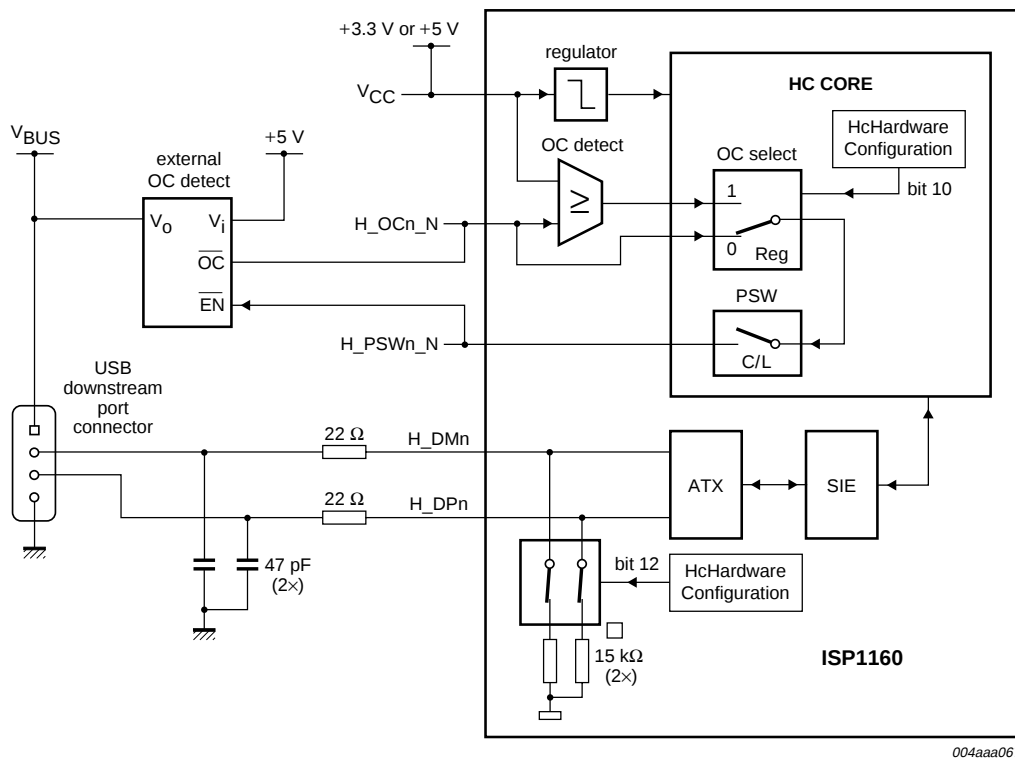
Fig 27. Using an external OC detection circuit.
