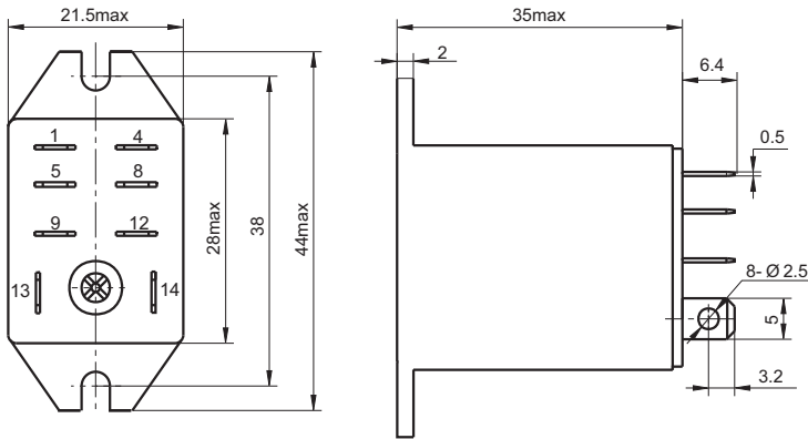
Outline Dimensions
