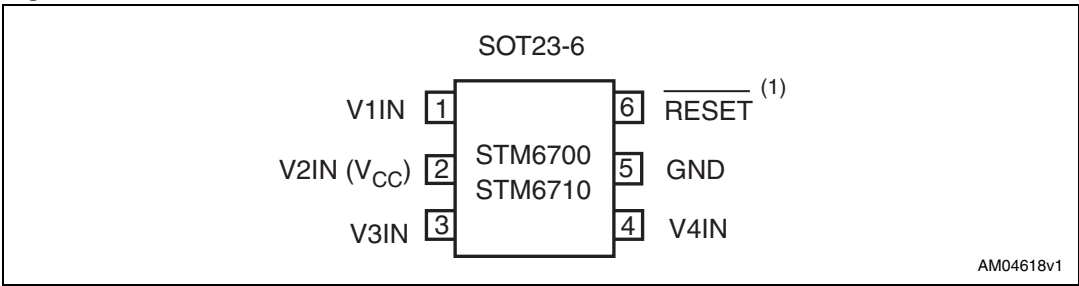
Figure 2. Pinout SOT23-6
