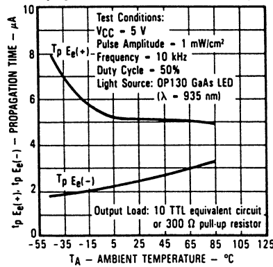
Propagation Time vs. Amb. Temp.
