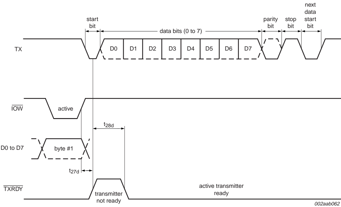
Fig 14. Transmit ready timing in non-FIFO mode
