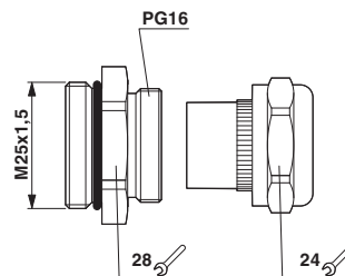
Dimensioned drawing
