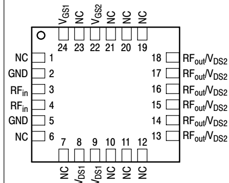
Figure 2. Pin Connections
