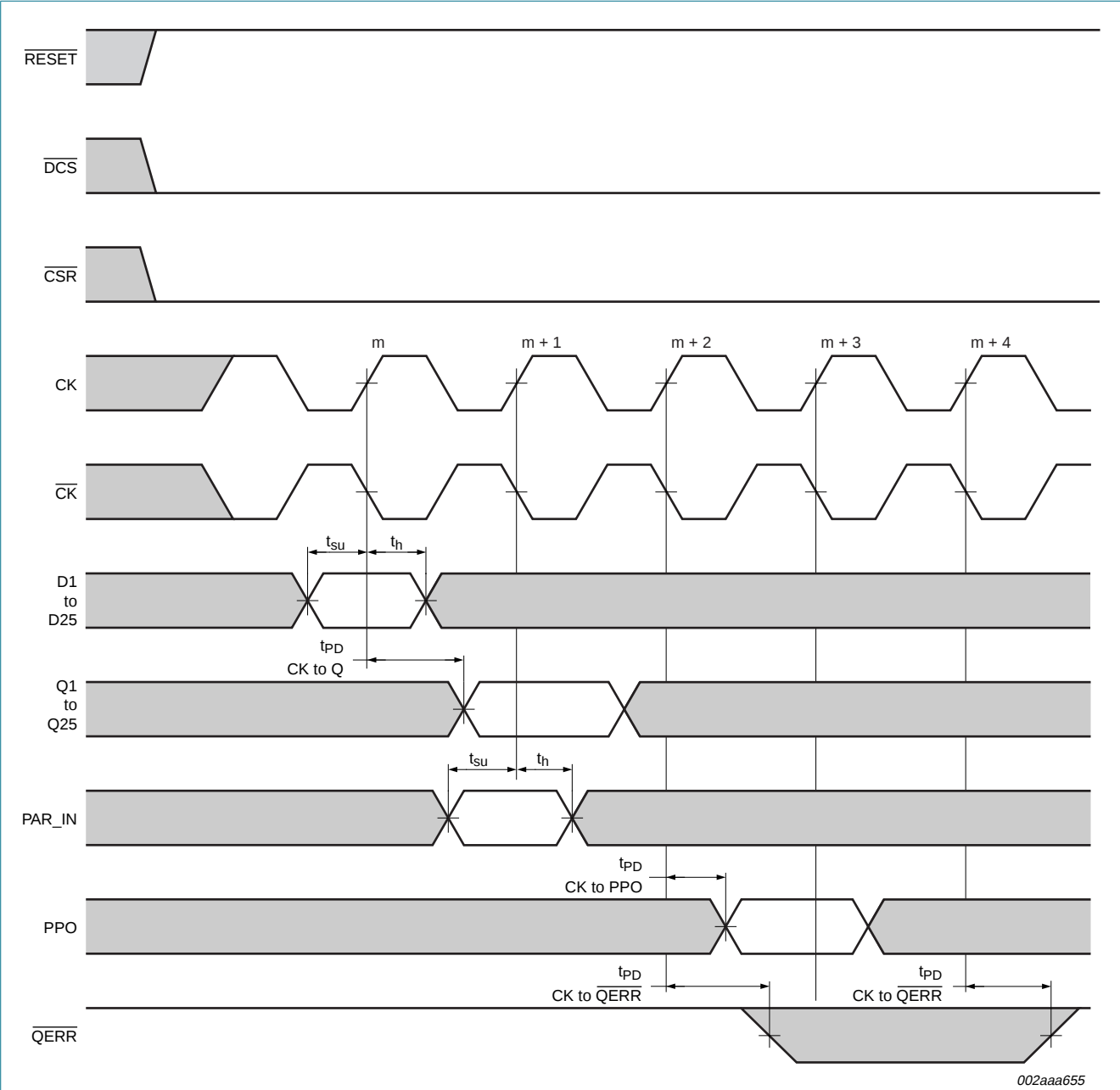
Fig 7. Timing diagram for SSTUG32866 used as a single device; C0 = 0, C1 = 0
