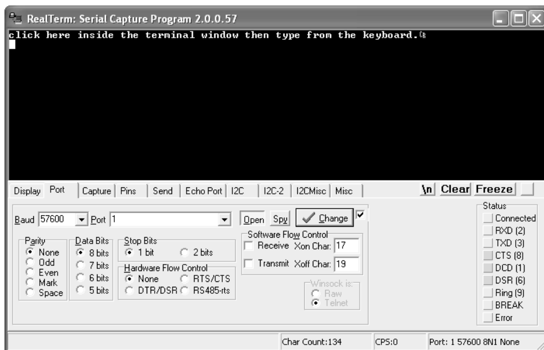
Figure 1. RealTerm Software Main Window (Port Tab Sheet)
