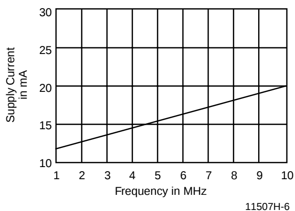
Figure 1. Typical Supply Current vs. Frequency V_{CC} = 5.5\ V , T = 25^{\circ}C
