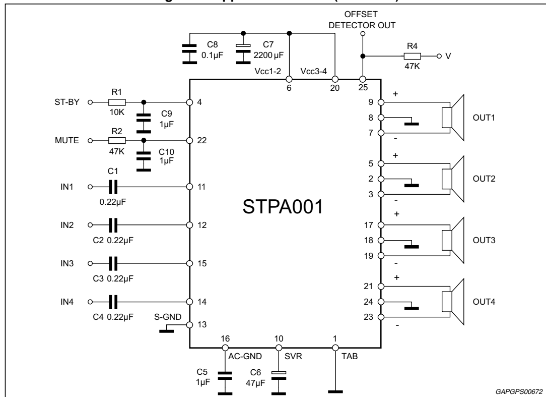
Figure 3. Application circuit (STPA001A &amp; STPA001H)
