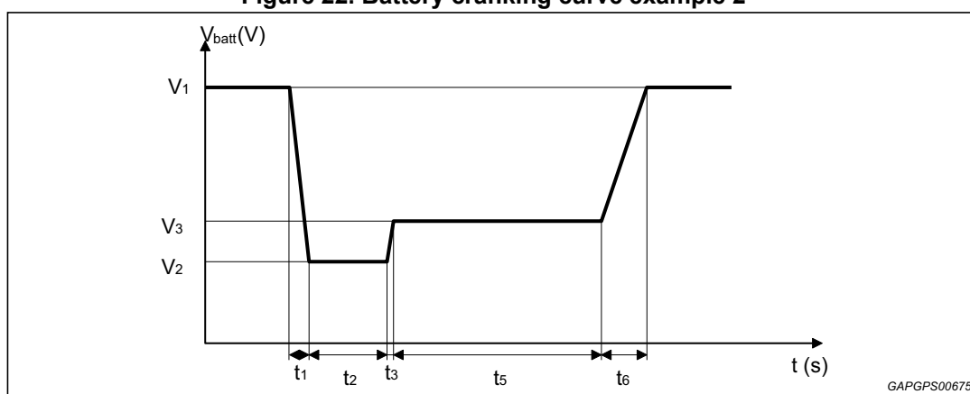
Figure 22. Battery cranking curve example 2
