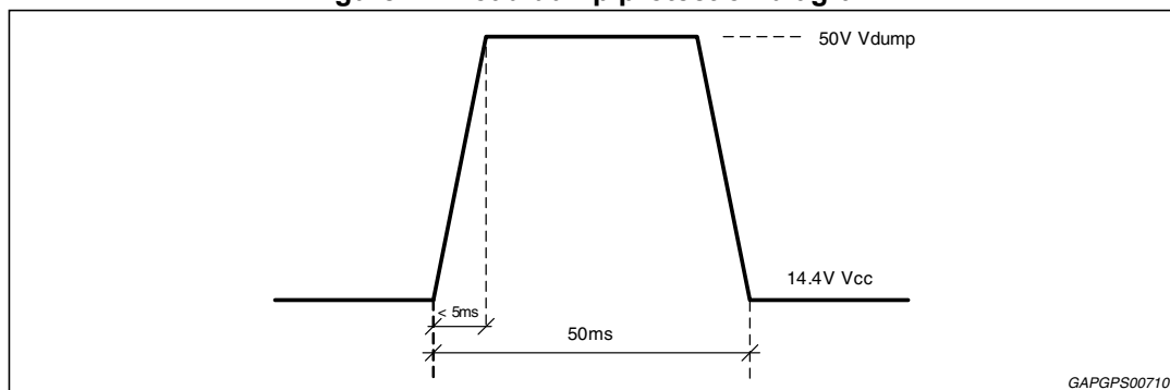
Figure 24. Load dump protection diagram
