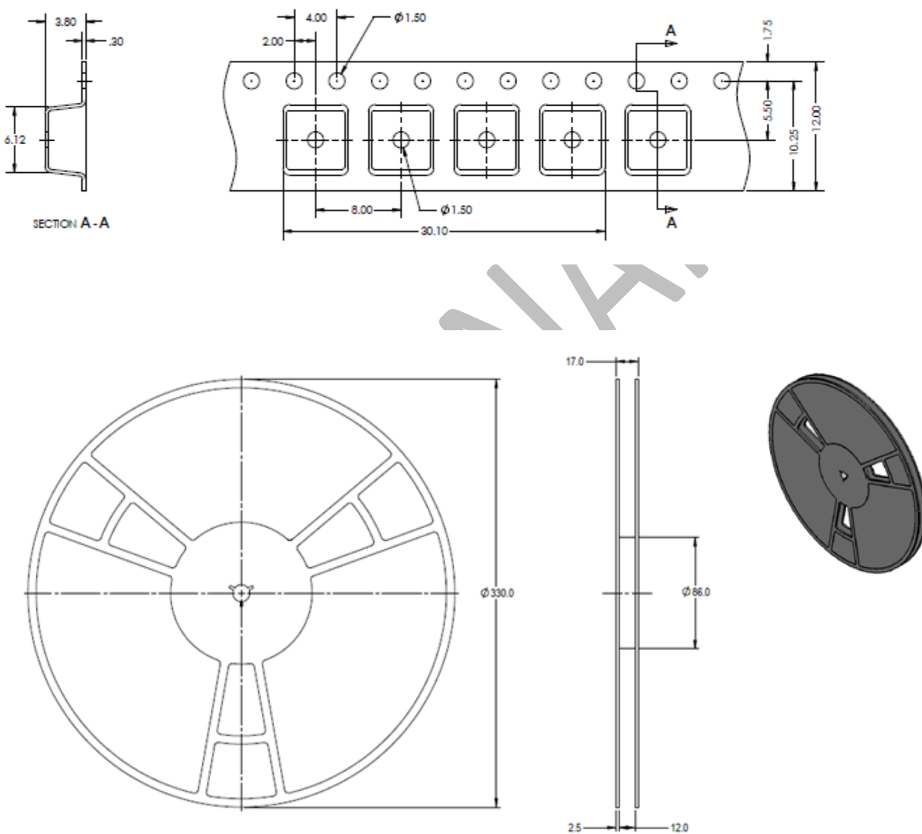
Figure 16: Tape and Reel Dimensions
