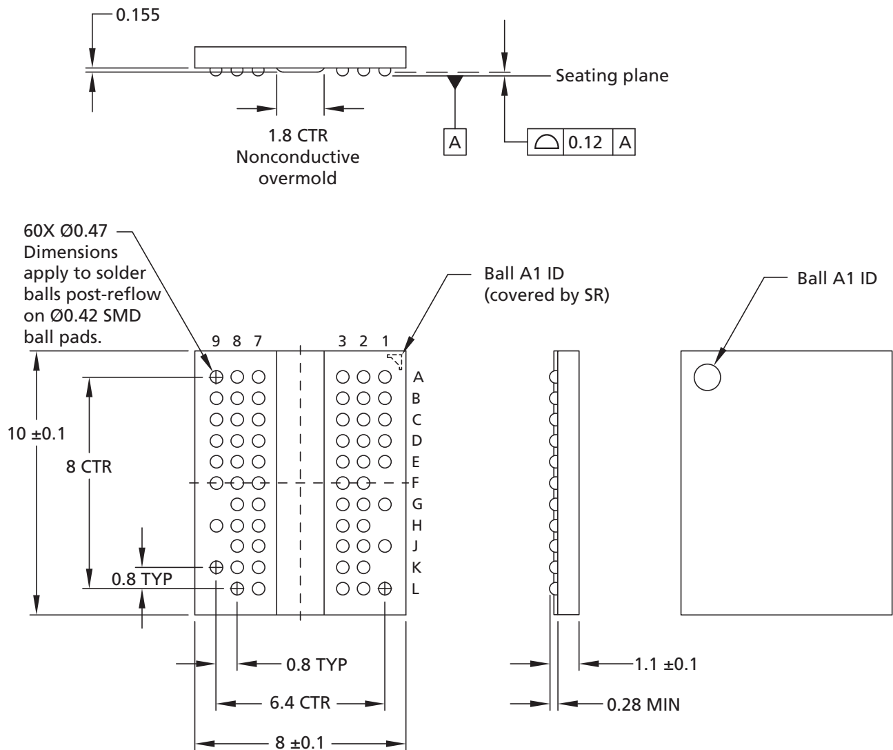
Figure 11: 60-Ball FBGA (8mm x 10mm) – x4, x8; "SH" Die Rev. :H
