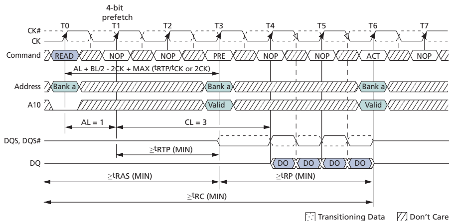
Figure 51: READ-to-PRECHARGE – BL = 4
