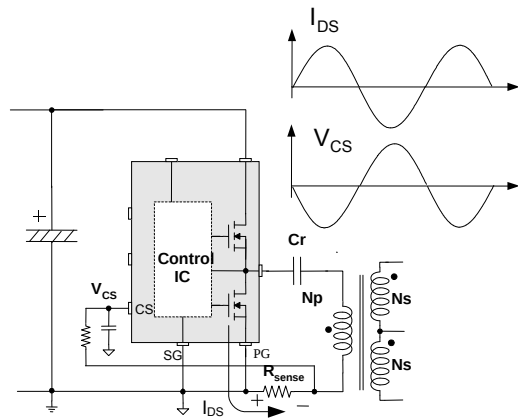
Figure 28. Full-Wave Sensing
