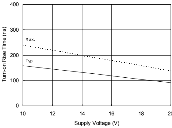
Figure 8B. Turn-on Rise Time vs. Supply Voltage
