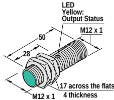
Classic Series NJ2-12GM40-E2-V1
