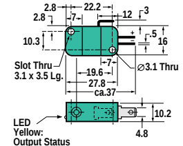
Basic Series NBB2-V3-E0-V5 NBB2-V3-E2-V5
