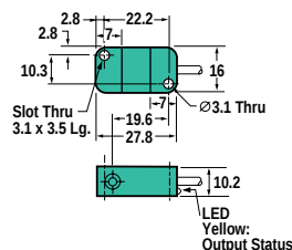
Basic Series NBB2-V3-E0 NBB2-V3-E2
