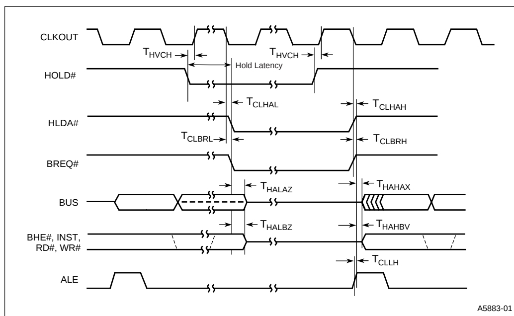
Figure 17. HOLD Timings
