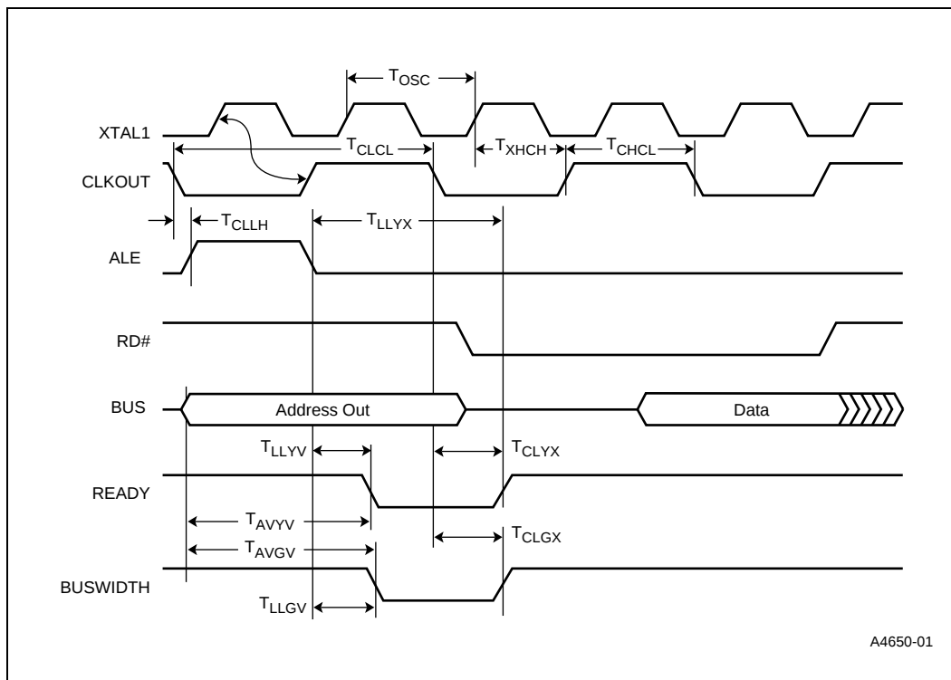
Figure 10. READY/Buswidth Timing
