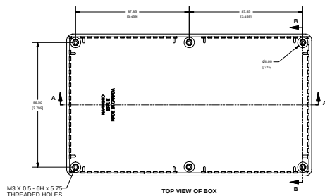
TOP VIEW OF BOX
