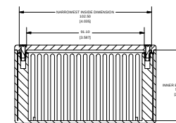
SECTION D-D SCALE 3/4
