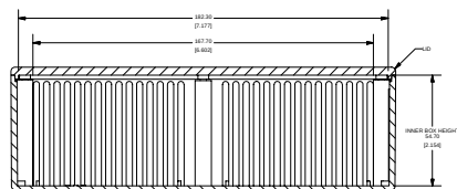
SECTION C-C SCALE 3/4
