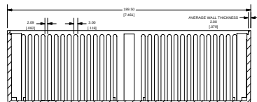
SECTION A-A SCALE 3/4
